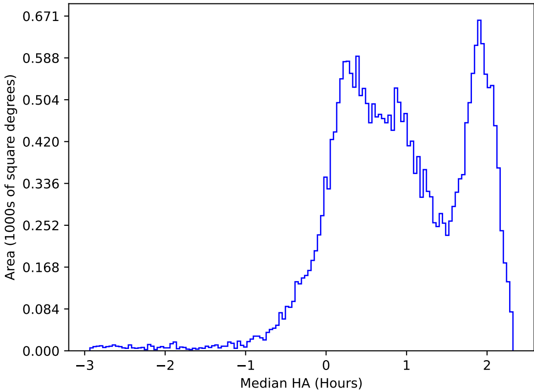
ddf_acor_sf10_lsf30_lsr20_v3.4_10yrs All sky i band: Median HA
