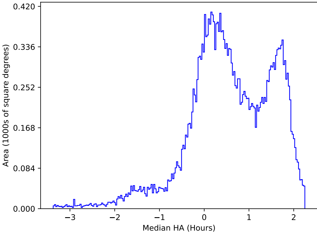
ddf_acor_sf10_lsf30_lsr20_v3.4_10yrs All sky g band: Median HA
