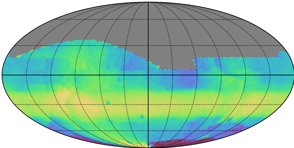
ddf_acor_sf10_lsf30_lsr20_v3.4_10yrs All sky all bands: Median HA
