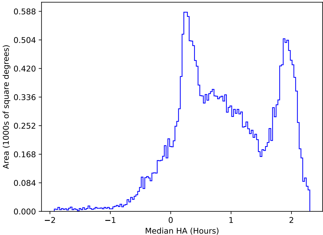
ddf_acor_sf10_lsf30_lsr20_v3.4_10yrs All sky all bands: Median HA
