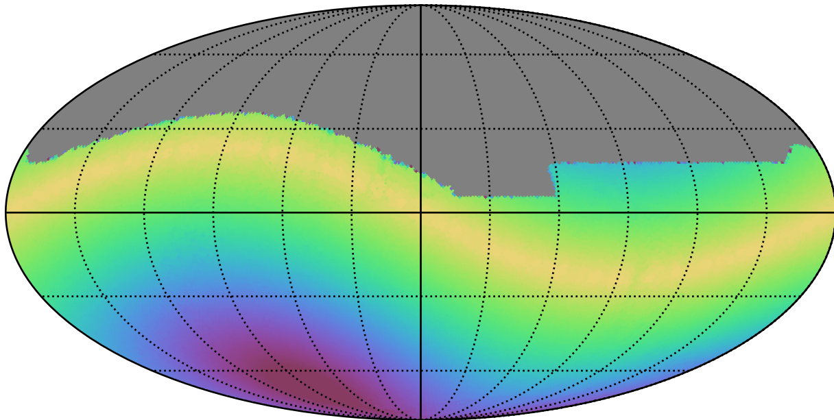
ddf_acor_sf10_lsf30_lsr20_v3.4_10yrs All sky i band: Max solarElong
