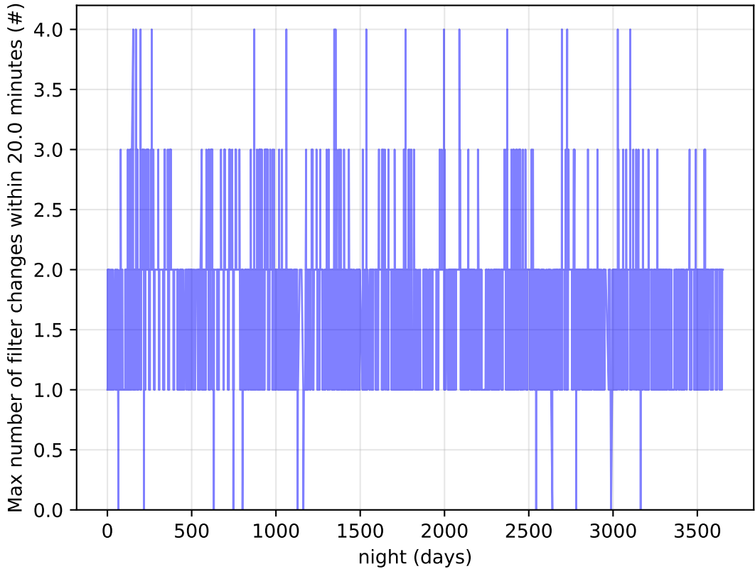
ddf_acor_sf10_Isf30_Isr20_v3.4_10yrs Per Night: Max number of filter changes within 20.0 minutes
