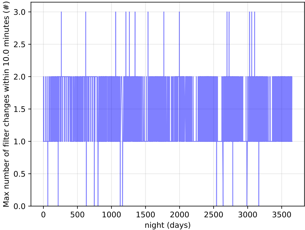
ddf_acor_sf10_Isf30_Isr20_v3.4_10yrs Per Night: Max number of filter changes within 10.0 minutes
