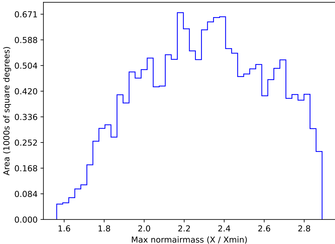
ddf_acor_sf10_lsf30_lsr20_v3.4_10yrs WFD z band: Max normairmass
