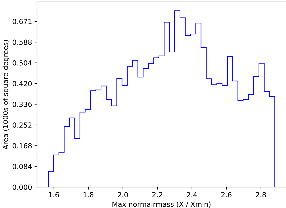
ddf_acor_sf10_lsf30_lsr20_v3.4_10yrs WFD i band: Max normairmass
