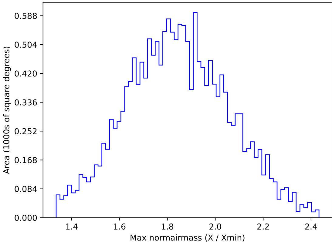
ddf_acor_sf10_lsf30_lsr20_v3.4_10yrs WFD g band: Max normairmass
