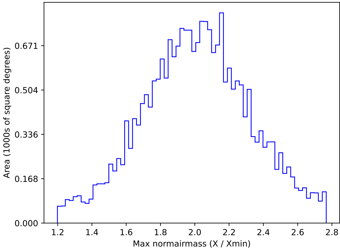
ddf_acor_sf10_lsf30_lsr20_v3.4_10yrs All sky y band: Max normairmass
