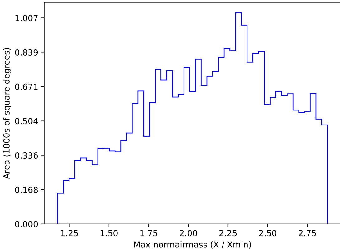
ddf_acor_sf10_lsf30_lsr20_v3.4_10yrs All sky i band: Max normairmass
