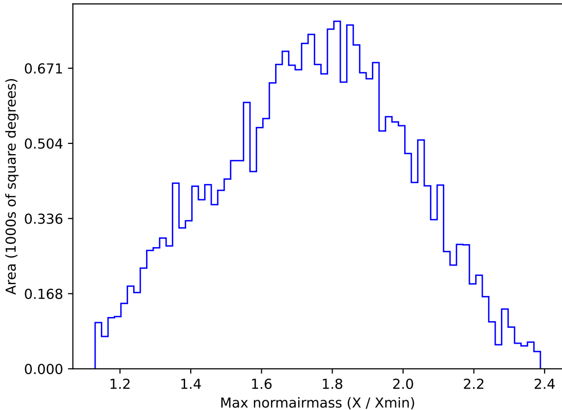
ddf_acor_sf10_lsf30_lsr20_v3.4_10yrs All sky g band: Max normairmass
