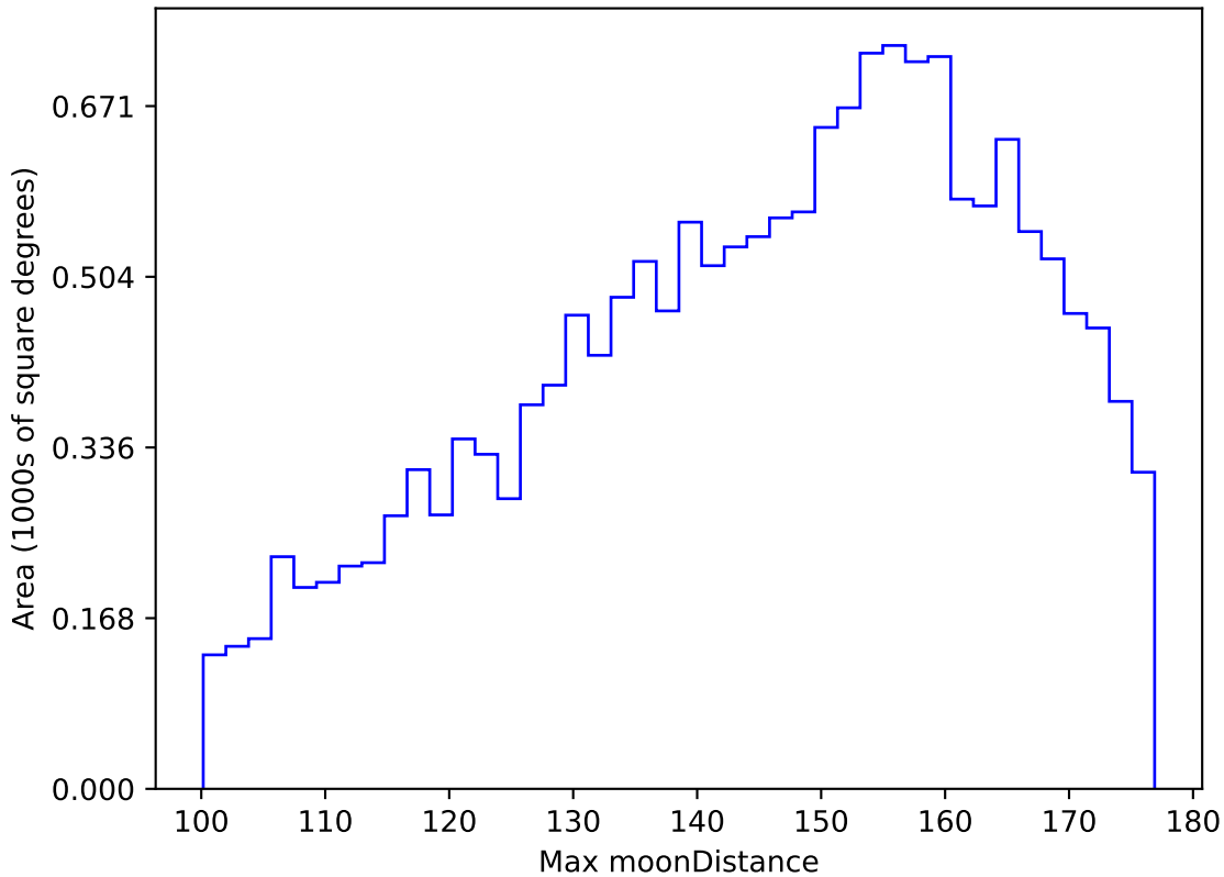
ddf_acor_sf10_lsf30_lsr20_v3.4_10yrs WFD y band: Max moonDistance
