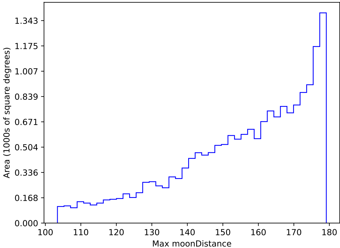
ddf_acor_sf10_lsf30_lsr20_v3.4_10yrs WFD i band: Max moonDistance
