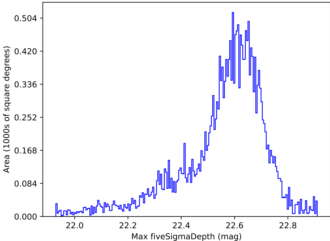
ddf_acor_sf10_ls30_lsr20_v3.4_10yrs All sky y band: Max fiveSigmaDepth
