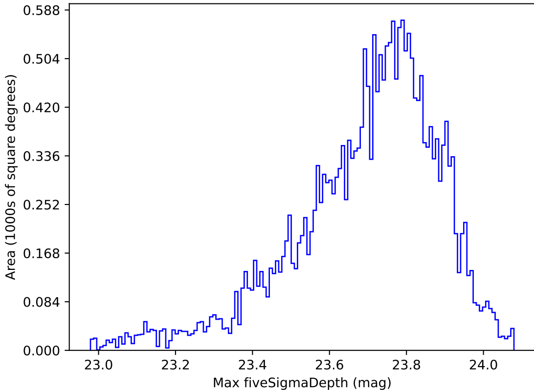
ddf_acor_sf10_lsf30_lsr20_v3.4_10yrs All sky u band: Max fiveSigmaDepth
