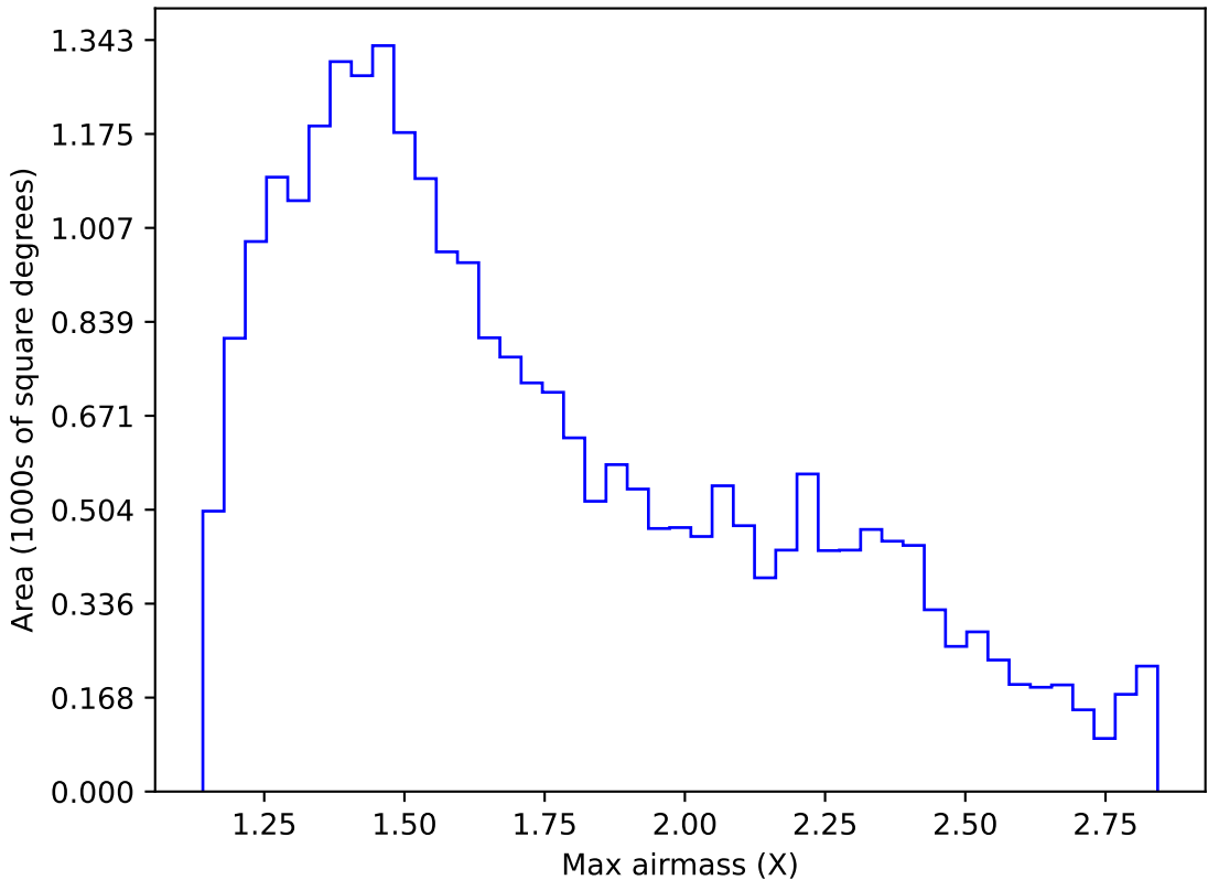
ddf_acor_sf10_lsf30_lsr20_v3.4_10yrs Yr 1 z band: Max airmass
