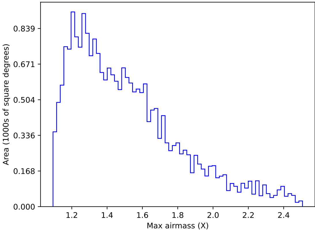
ddf_acor_sf10_lsf30_lsr20_v3.4_10yrs Yr 1 u band: Max airmass
