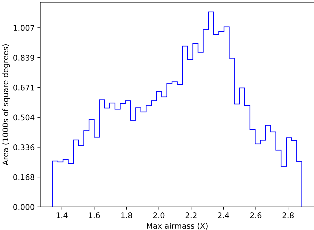
ddf_acor_sf10_lsf30_lsr20_v3.4_10yrs Yr 1 all bands: Max airmass
