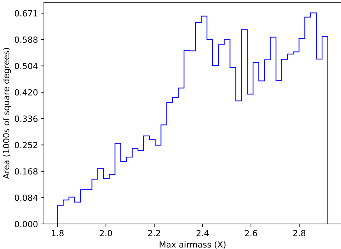
ddf_acor_sf10_lsf30_lsr20_v3.4_10yrs WFD z band: Max airmass
