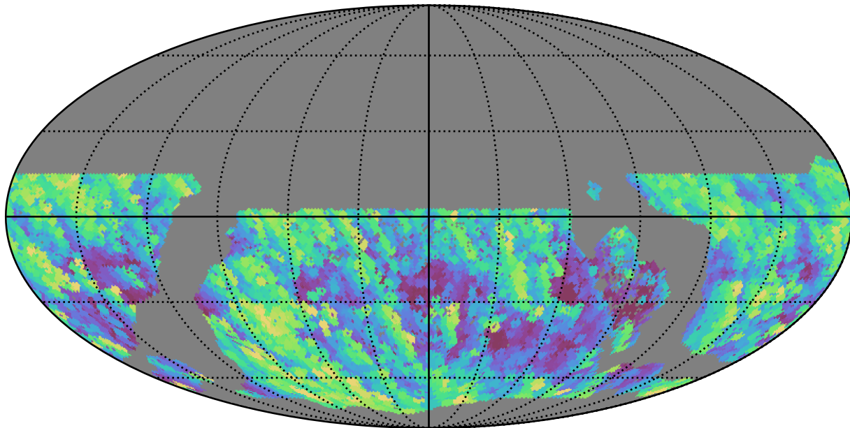
ddf_acor_sf10_lsf30_lsr20_v3.4_10yrs WFD y band: Max airmass
