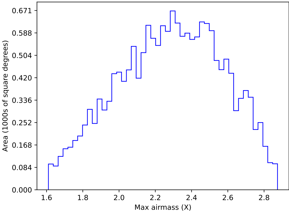
ddf_acor_sf10_lsf30_lsr20_v3.4_10yrs WFD y band: Max airmass
