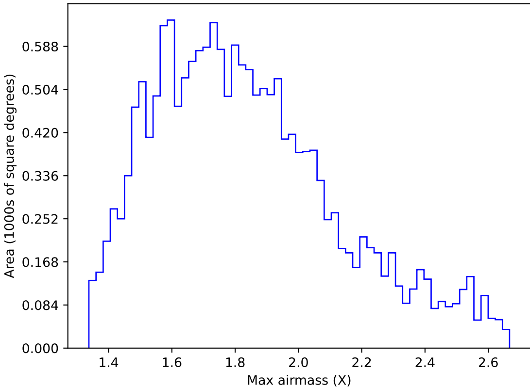
ddf_acor_sf10_ls30_lsr20_v3.4_10yrs WFD u band: Max airmass
