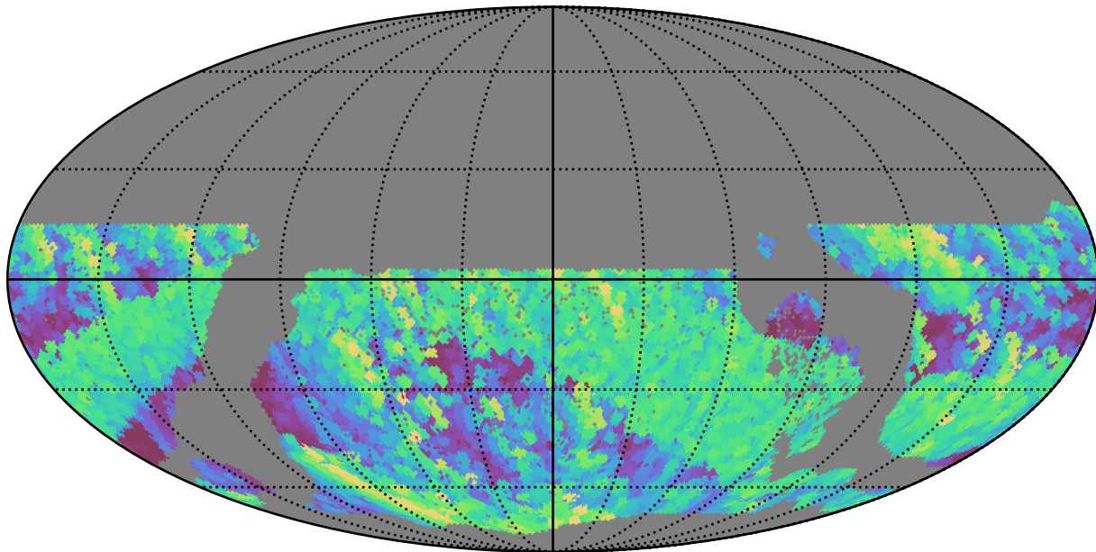
ddf_acor_sf10_lsf30_lsr20_v3.4_10yrs WFD r band: Max airmass
