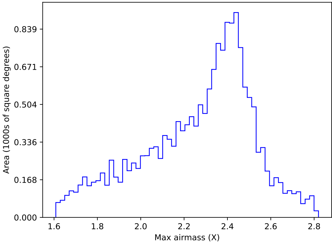
ddf_acor_sf10_ls30_lsr20_v3.4_10yrs WFD r band: Max airmass
