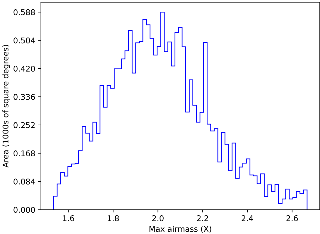
ddf_acor_sf10_ls30_lsr20_v3.4_10yrs WFD g band: Max airmass
