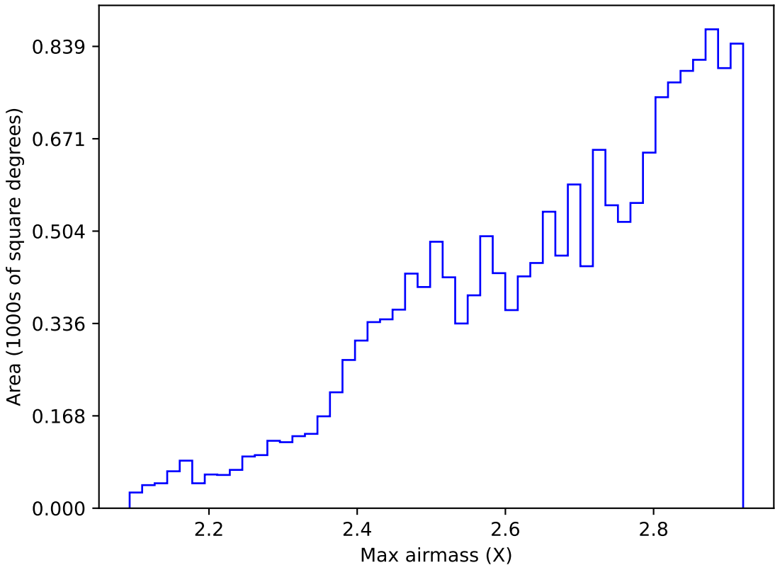
ddf_acor_sf10_lsf30_lsr20_v3.4_10yrs WFD all bands: Max airmass
