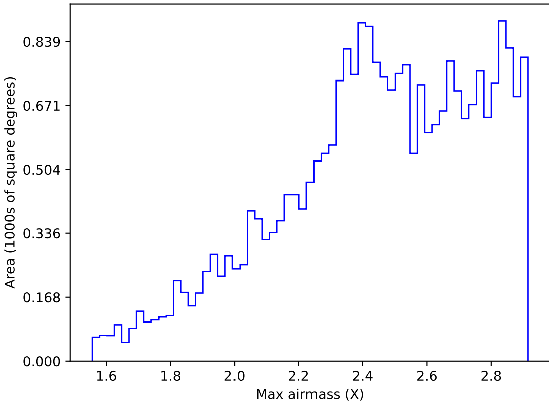
ddf_acor_sf10_lsf30_lsr20_v3.4_10yrs All sky z band: Max airmass
