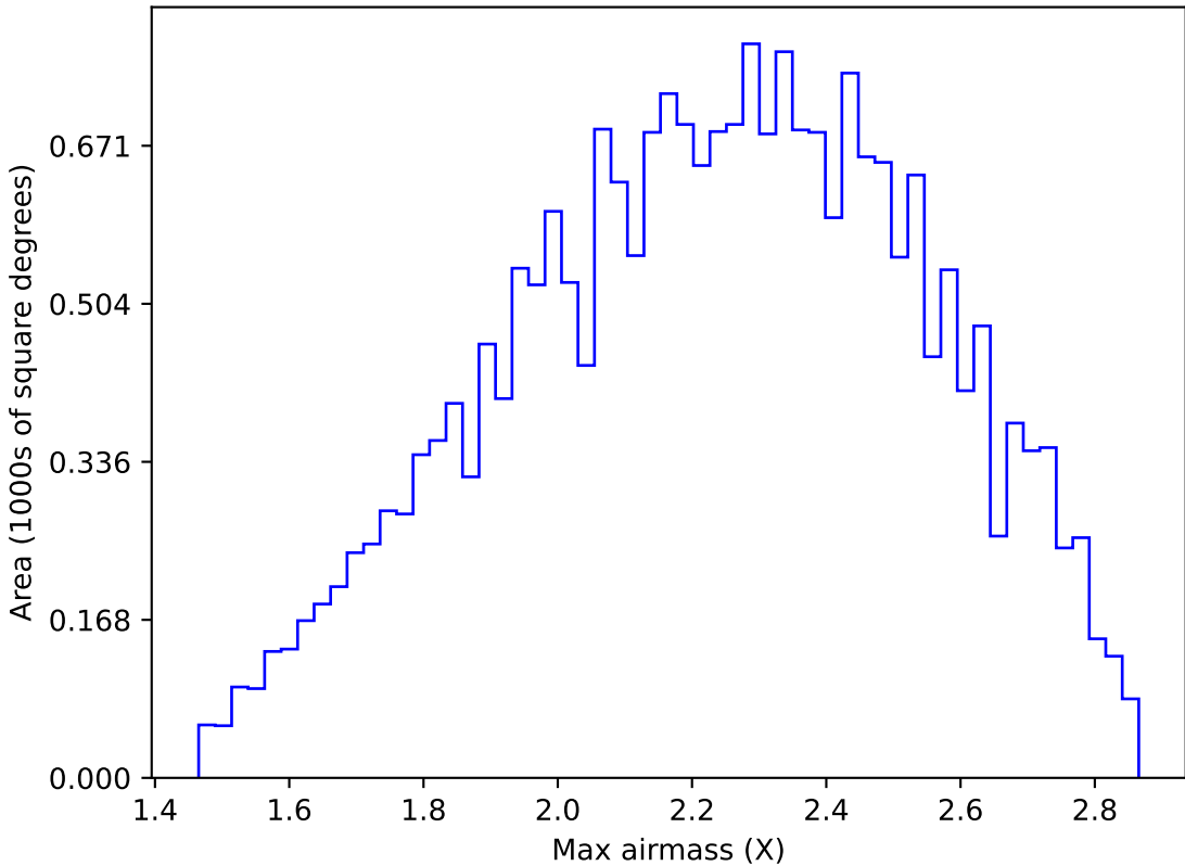
ddf_acor_sf10_lsf30_lsr20_v3.4_10yrs All sky y band: Max airmass
