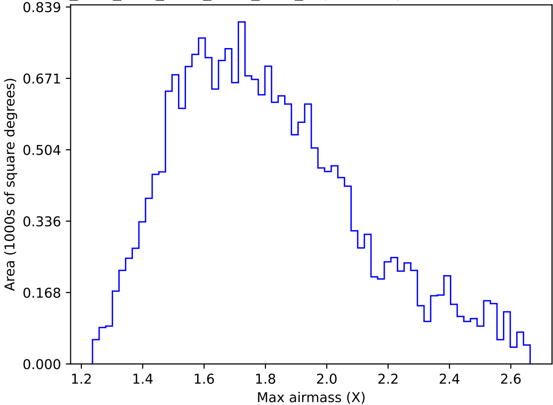
ddf_acor_sf10_lsf30_lsr20_v3.4_10yrs All sky u band: Max airmass
