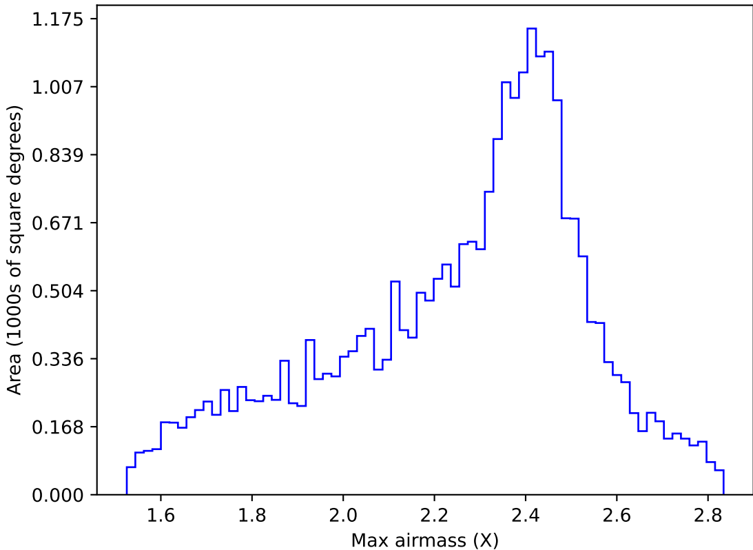
ddf_acor_sf10_lsf30_lsr20_v3.4_10yrs All sky r band: Max airmass
