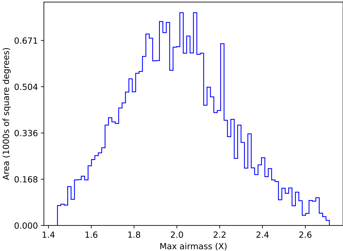
ddf_acor_sf10_lsf30_lsr20_v3.4_10yrs All sky g band: Max airmass
