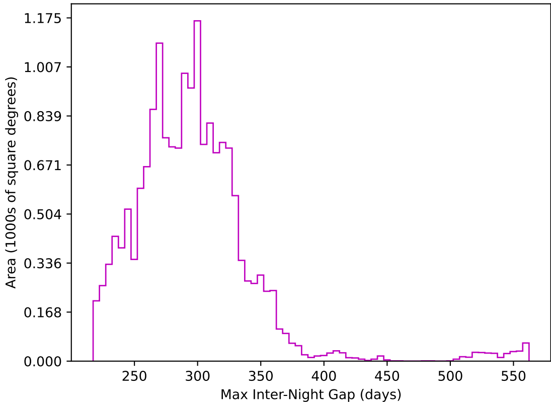
ddf_acor_sf10_lsf30_lsr20_v3.4_10yrs WFD z band: Max Inter-Night Gap
