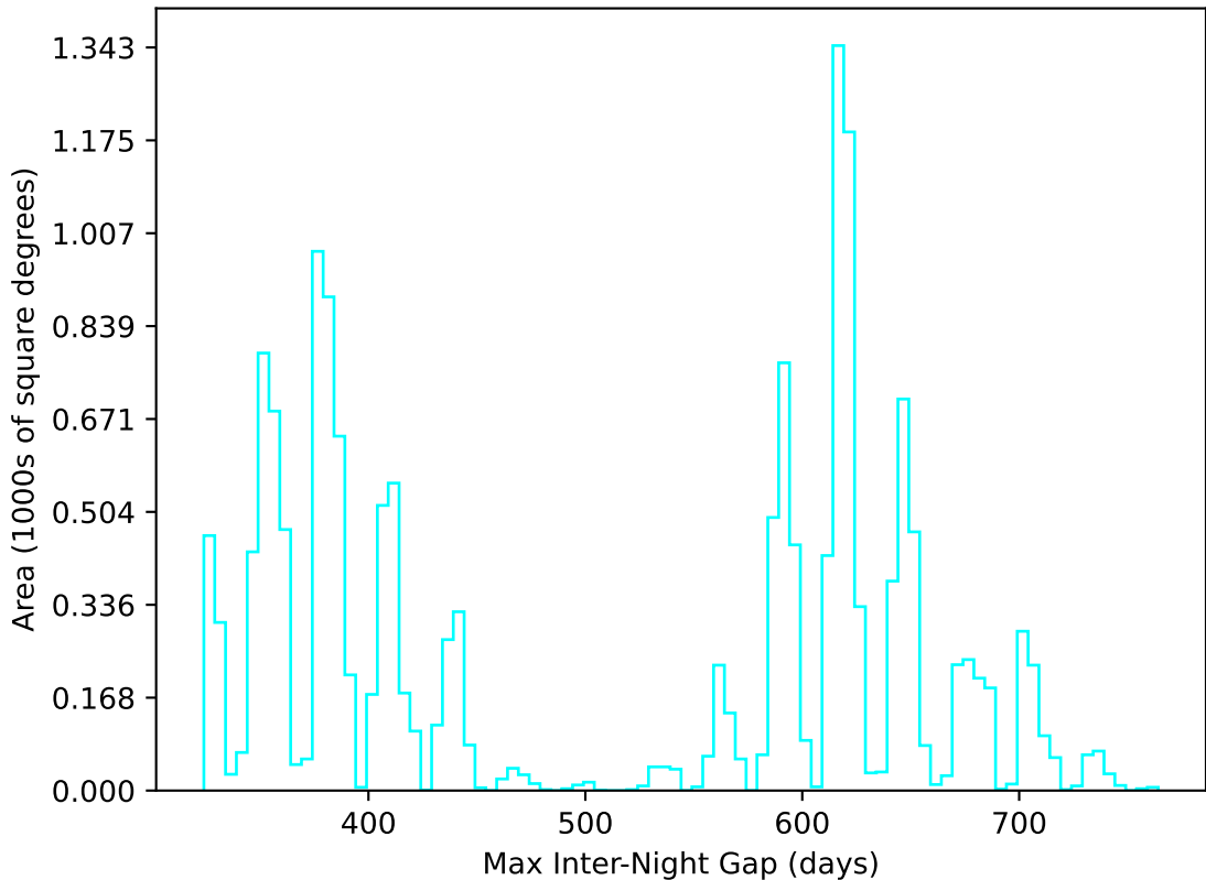
ddf_acor_sf10_lsf30_lsr20_v3.4_10yrs WFD u band: Max Inter-Night Gap
