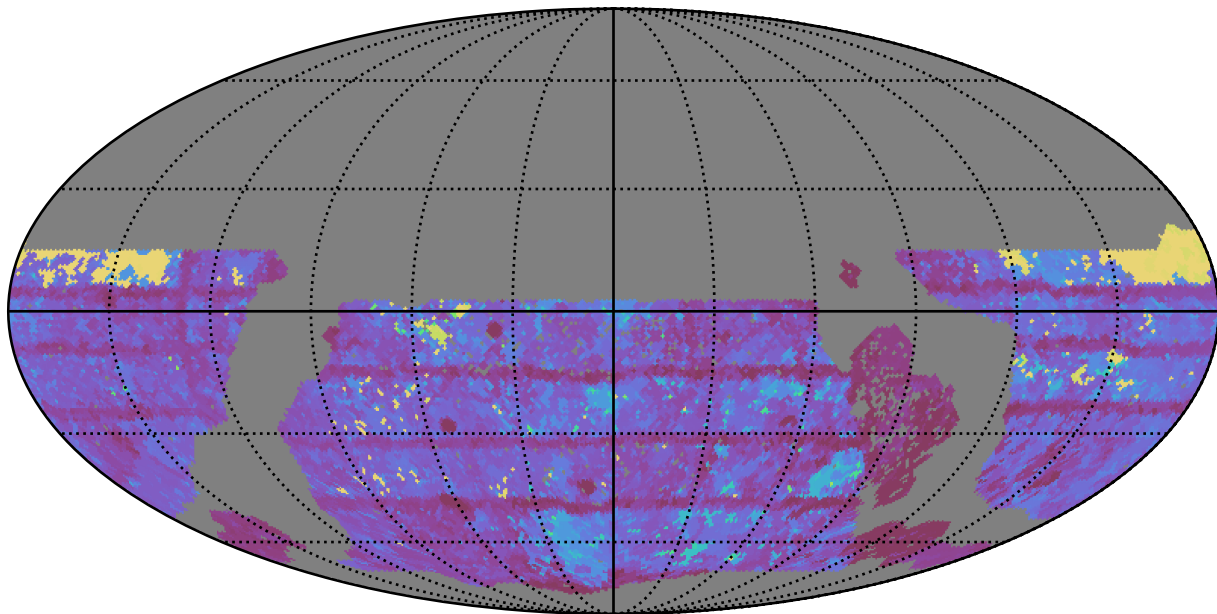
ddf_acor_sf10_lsf30_lsr20_v3.4_10yrs WFD r band: Max Inter-Night Gap
