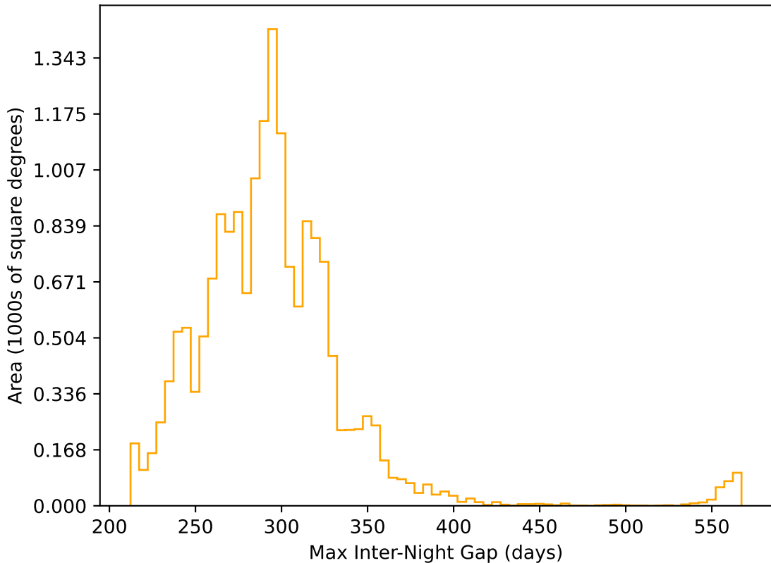
ddf_acor_sf10_lsf30_lsr20_v3.4_10yrs WFD r band: Max Inter-Night Gap
