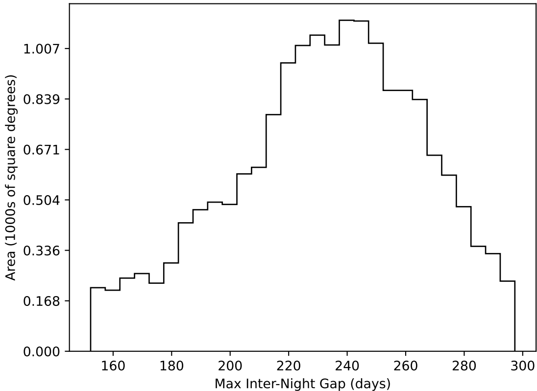
ddf_acor_sf10_lsf30_lsr20_v3.4_10yrs WFD all bands: Max Inter-Night Gap
