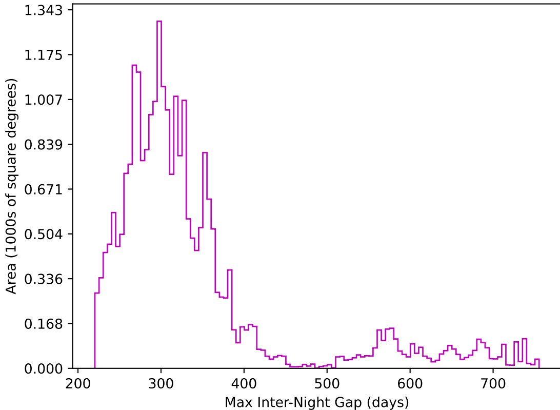
ddf_acor_sf10_lsf30_lsr20_v3.4_10yrs All sky z band: Max Inter-Night Gap
