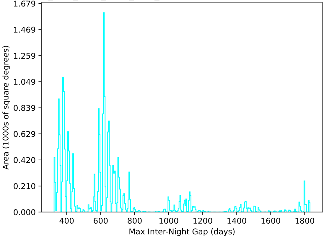
ddf_acor_sf10_lsf30_lsr20_v3.4_10yrs All sky u band: Max Inter-Night Gap
