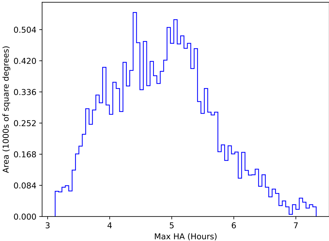
ddf_acor_sf10_lsf30_lsr20_v3.4_10yrs WFD i band: Max HA
