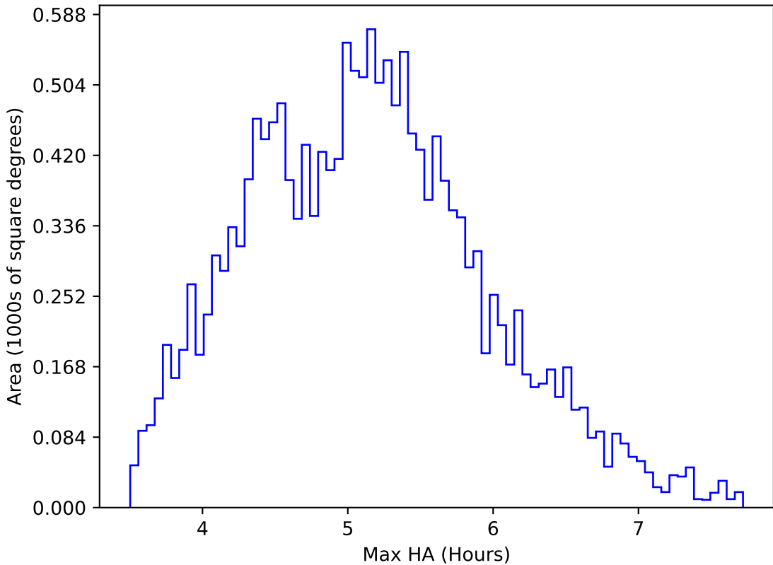
ddf_acor_sf10_lsf30_lsr20_v3.4_10yrs WFD all bands: Max HA
