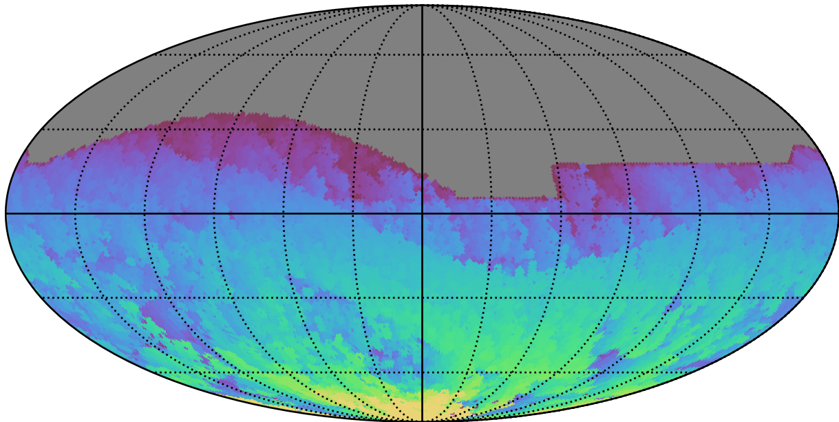
ddf_acor_sf10_lsf30_lsr20_v3.4_10yrs All sky z band: Max HA
