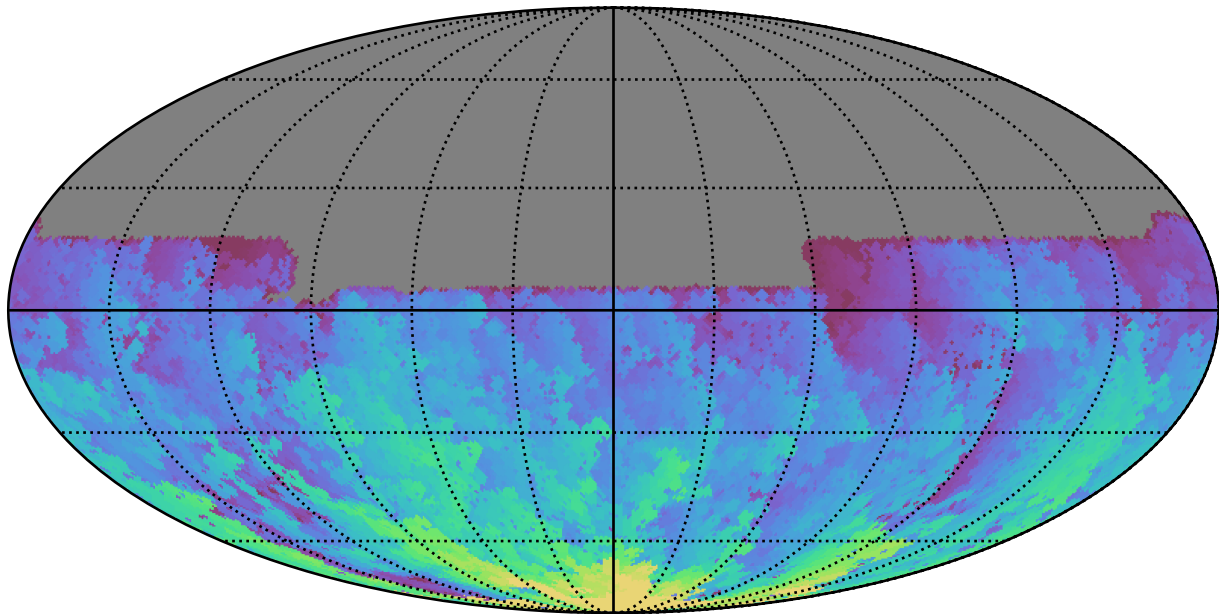
ddf_acor_sf10_lsf30_lsr20_v3.4_10yrs All sky u band: Max HA
