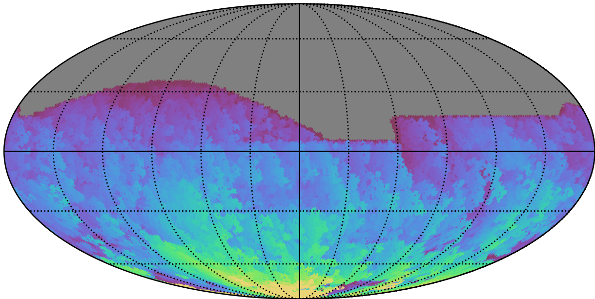
ddf_acor_sf10_lsf30_lsr20_v3.4_10yrs All sky r band: Max HA
