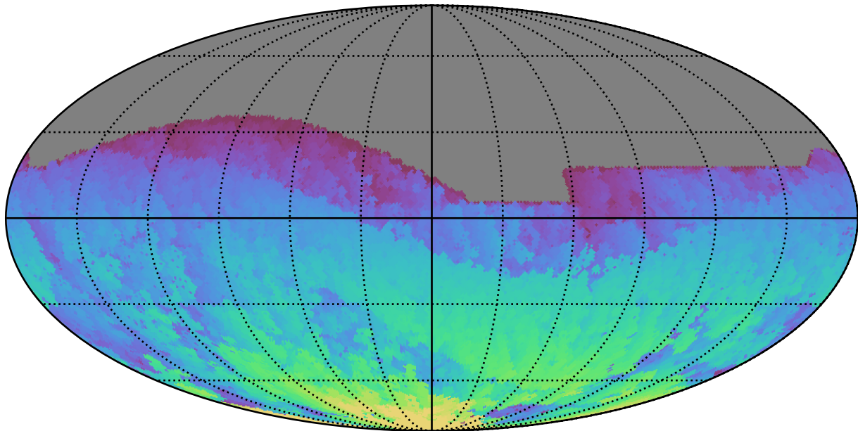
ddf_acor_sf10_lsf30_lsr20_v3.4_10yrs All sky i band: Max HA
