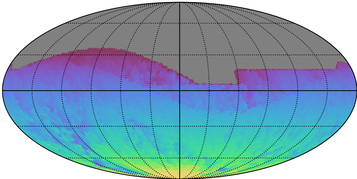
ddf_acor_sf10_lsf30_lsr20_v3.4_10yrs All sky all bands: Max HA
