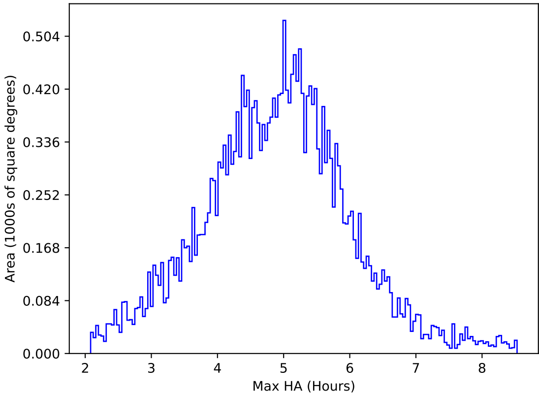
ddf_acor_sf10_lsf30_lsr20_v3.4_10yrs All sky all bands: Max HA
