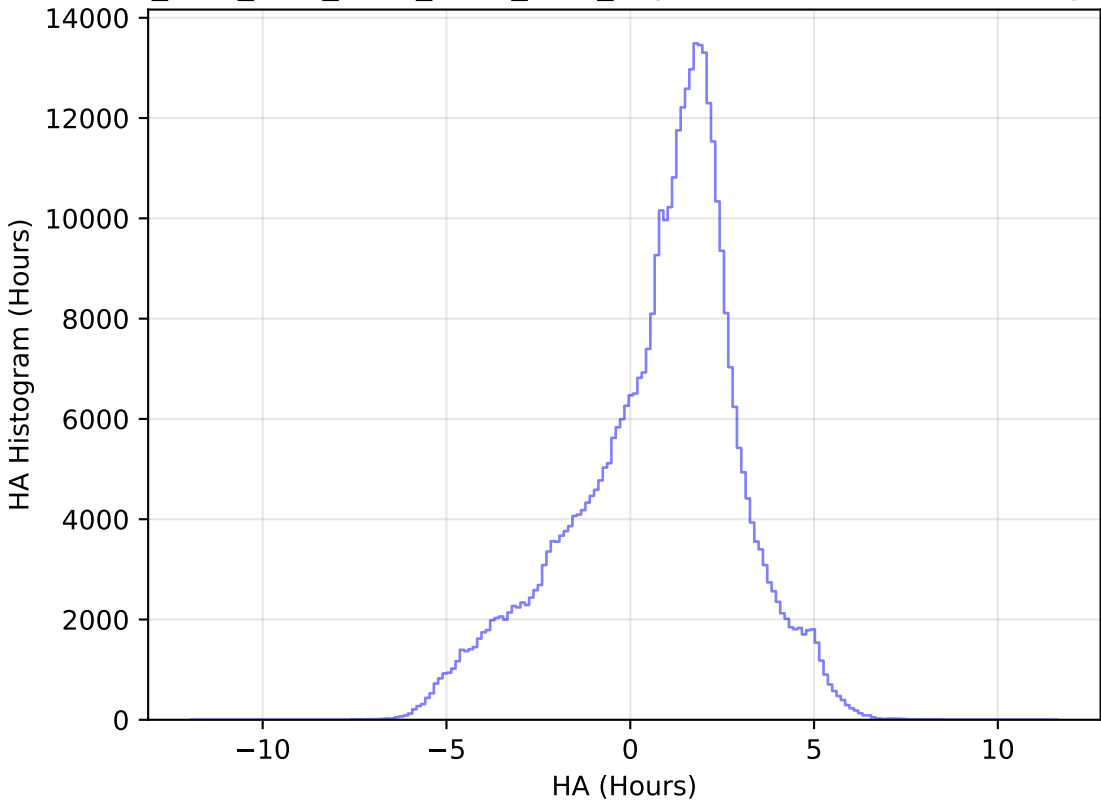
ddf_acor_sf10_lsf30_lsr20_v3.4_10yrs WFD z band: HA Histogram
