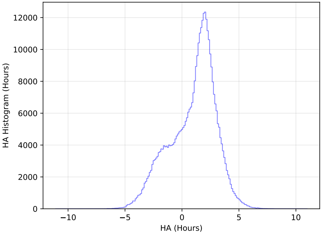
ddf_acor_sf10_lsf30_lsr20_v3.4_10yrs WFD y band: HA Histogram
